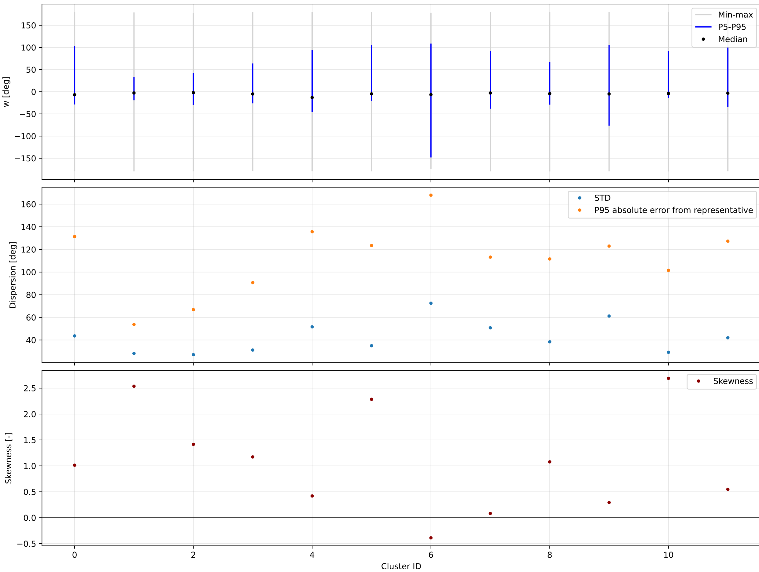
K=12 | forward | w | valid=194050/194058 | offsets from each cluster circular mean
