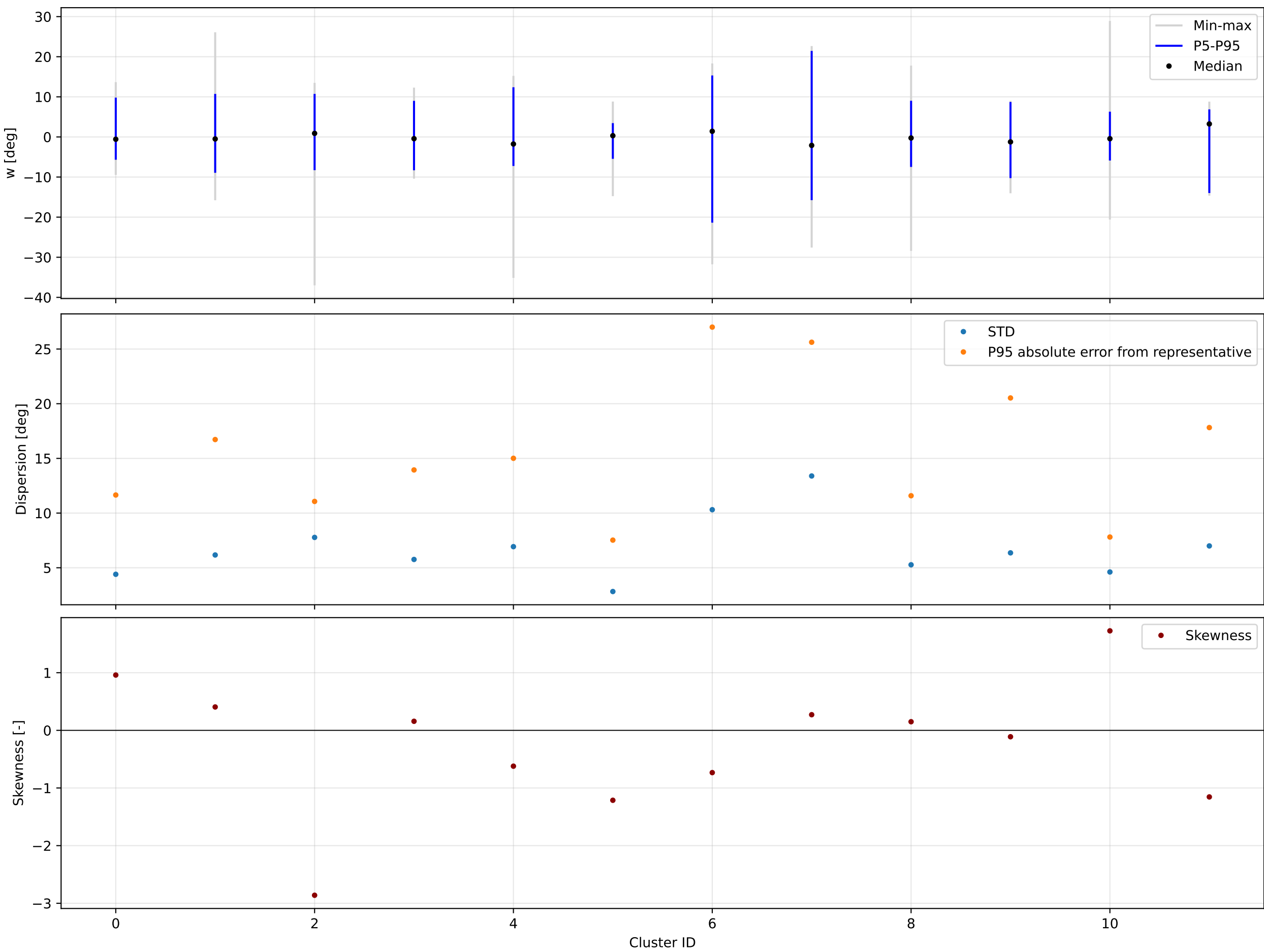
K=12 | backward | w | valid=194058/194058 | offsets from each cluster circular mean
