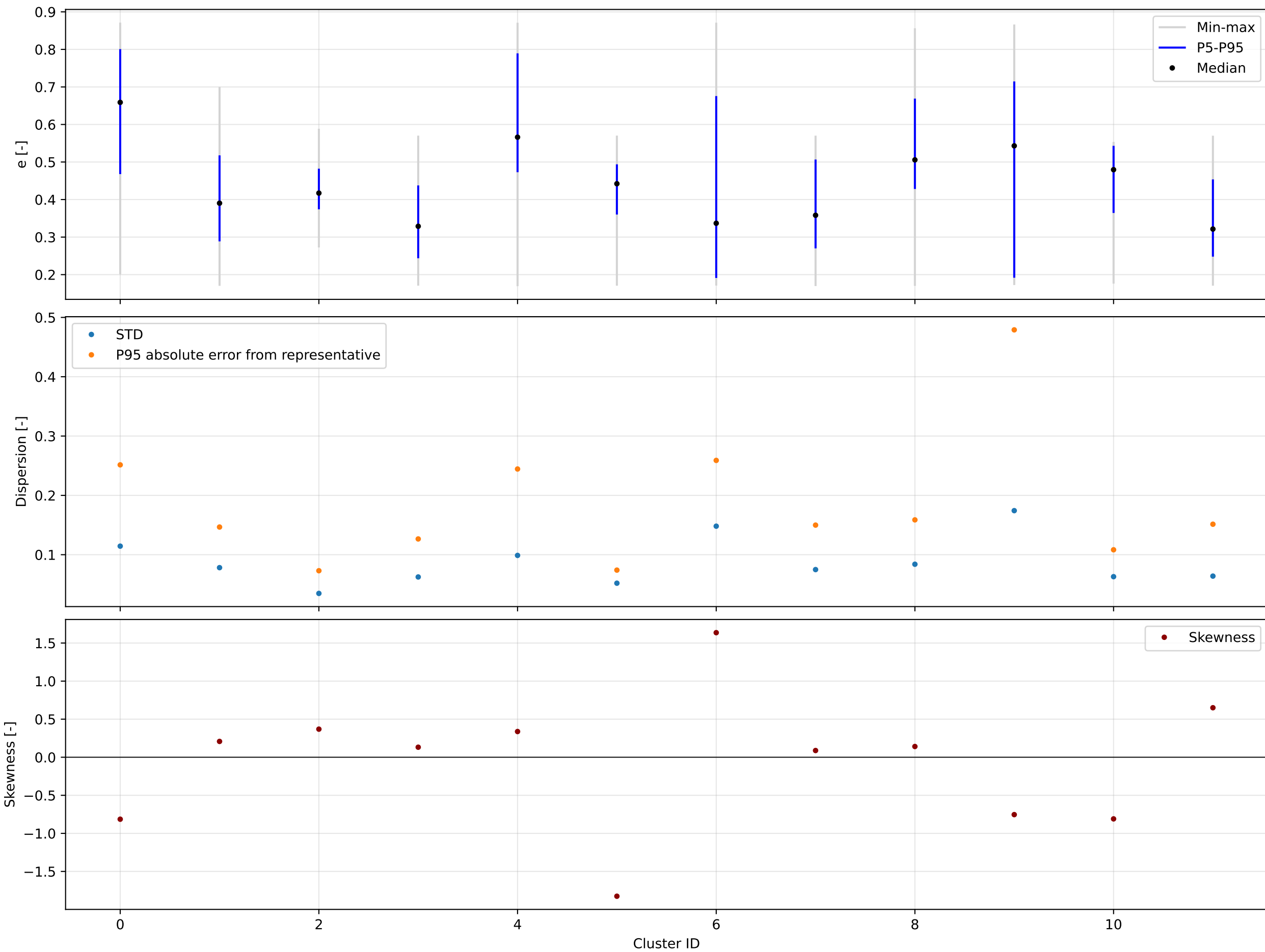
K=12 | forward | e | valid=194050/194058
